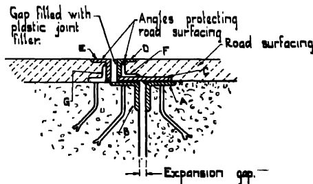
Fig. 337. —Expansion Joint in Deck Slab.
